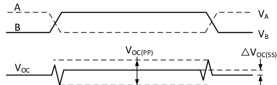
Figure 2. Measurement of Driver Differential and Common-Mode Output with RS-485 Load
